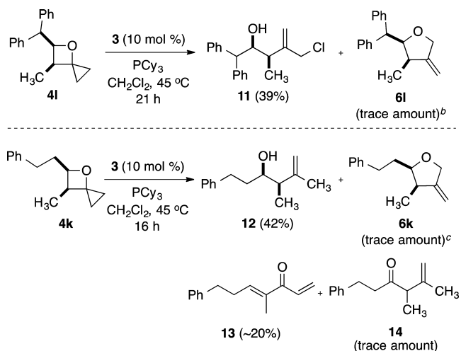
Scheme 1. Reaction of cis -5,6-Oxaspirohexanes with Zeise's Dimer a
