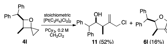
Scheme 6. Reaction of Oxaspirohexane 4l with a Stoichiometric Amount of Zeise's Dimer
