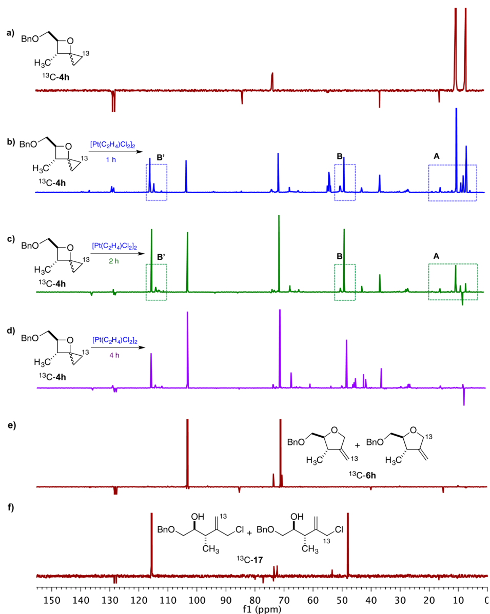
Figure 5. 13 C DEPT NMR monitoring of the reaction of 13 C-4h (0.1 mmol) with a stoichiometric amount of Zeise's dimer and PCy 3 and with 0.2 M 13 C-4h in CD 2 Cl 2 at RT. (a) 13 C DEPT NMR spectra of oxaspirohexanes 13 C-4h. (b) 13 C NMR spectrum after 1 h. (c) 13 C DEPT after 2 h. (d) 13 C DEPT NMR after 4 h. (e) 13 C DEPT of methylenetetrahydrofuran products 13 C-6h. (f) 13 C DEPT of allyl chloride byproducts 13 C-17.
